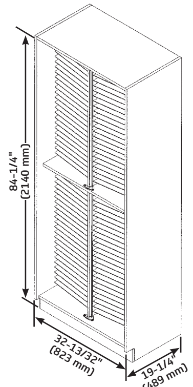
Band/Orchestra Folio Cabinet
