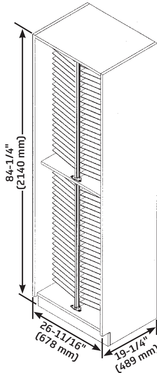
Choral Folio Cabinet
